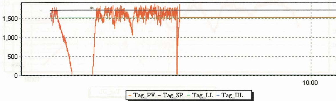
PV Trend for loop Calcine_Bed_Level_Control
