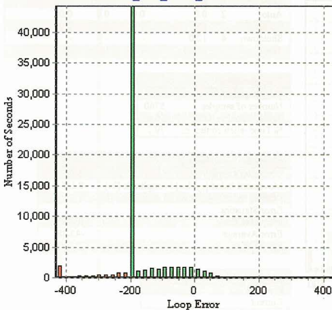
Error Histogram for Calcine_Bed_Level_Control
