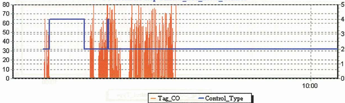
CO Trend for loop Calcine_Bed_Level_Control
